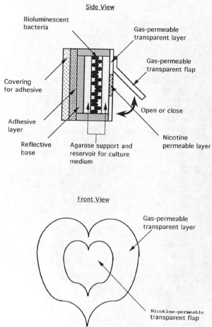
Fig. 1. Preliminary Design for a Nicotine-sensing Behavior Modification Device.
